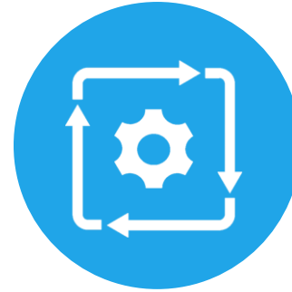
Iterative Design
